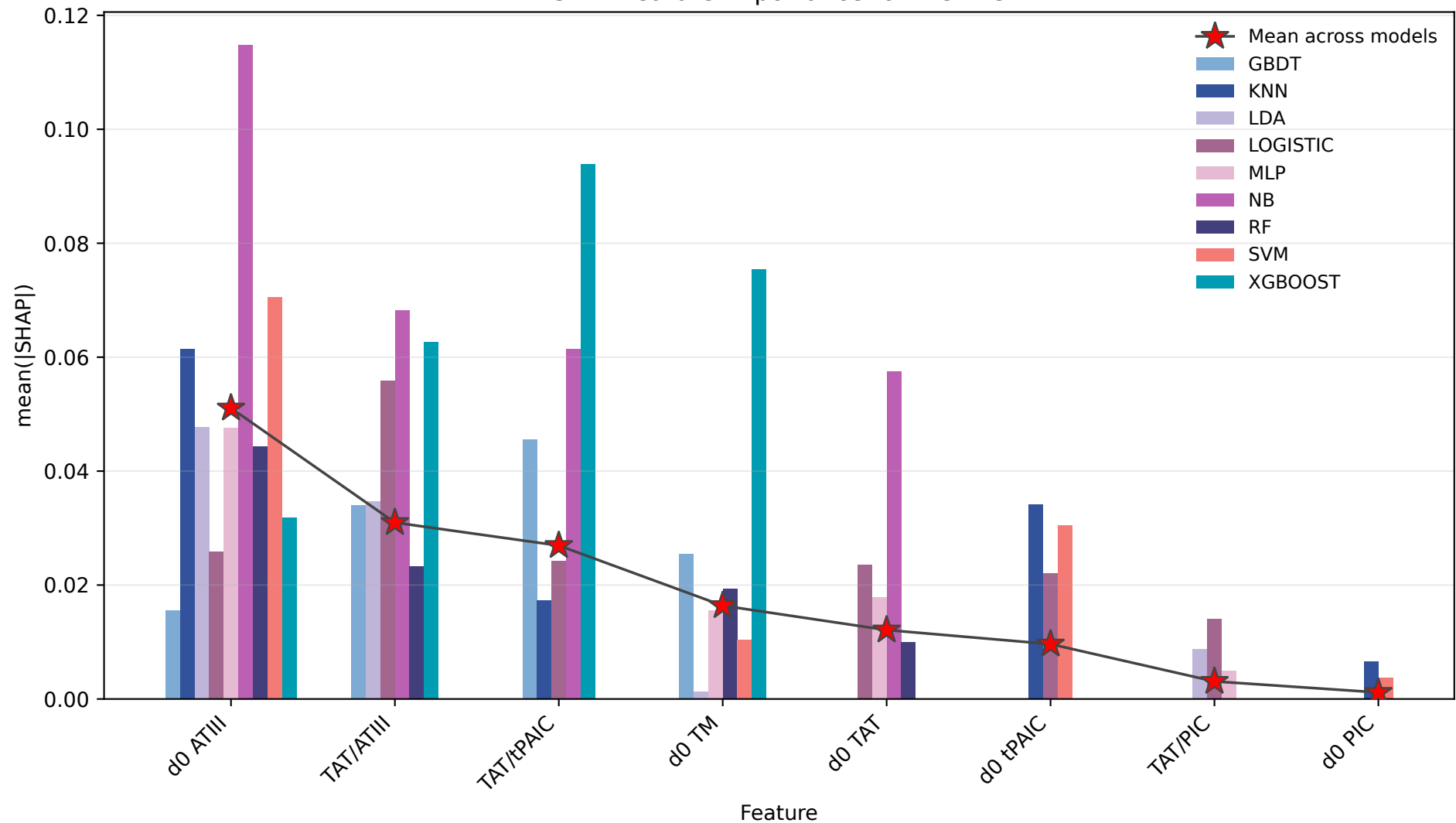
SHAP feature importance for Pre-DIC
